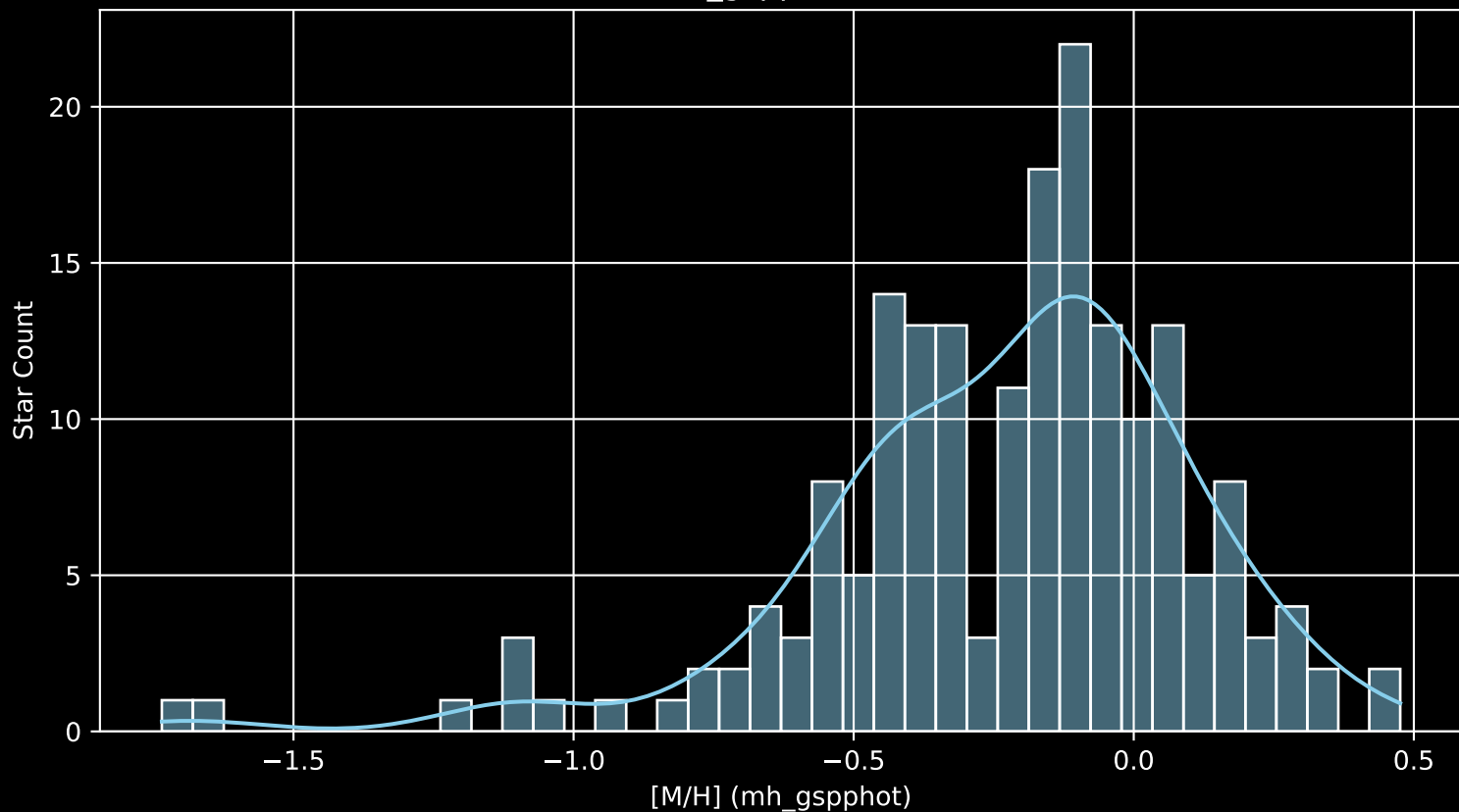
APOGEE DR17 Field: [137+79_MGA [M/H] (mh_gspphot) (n= 187)
