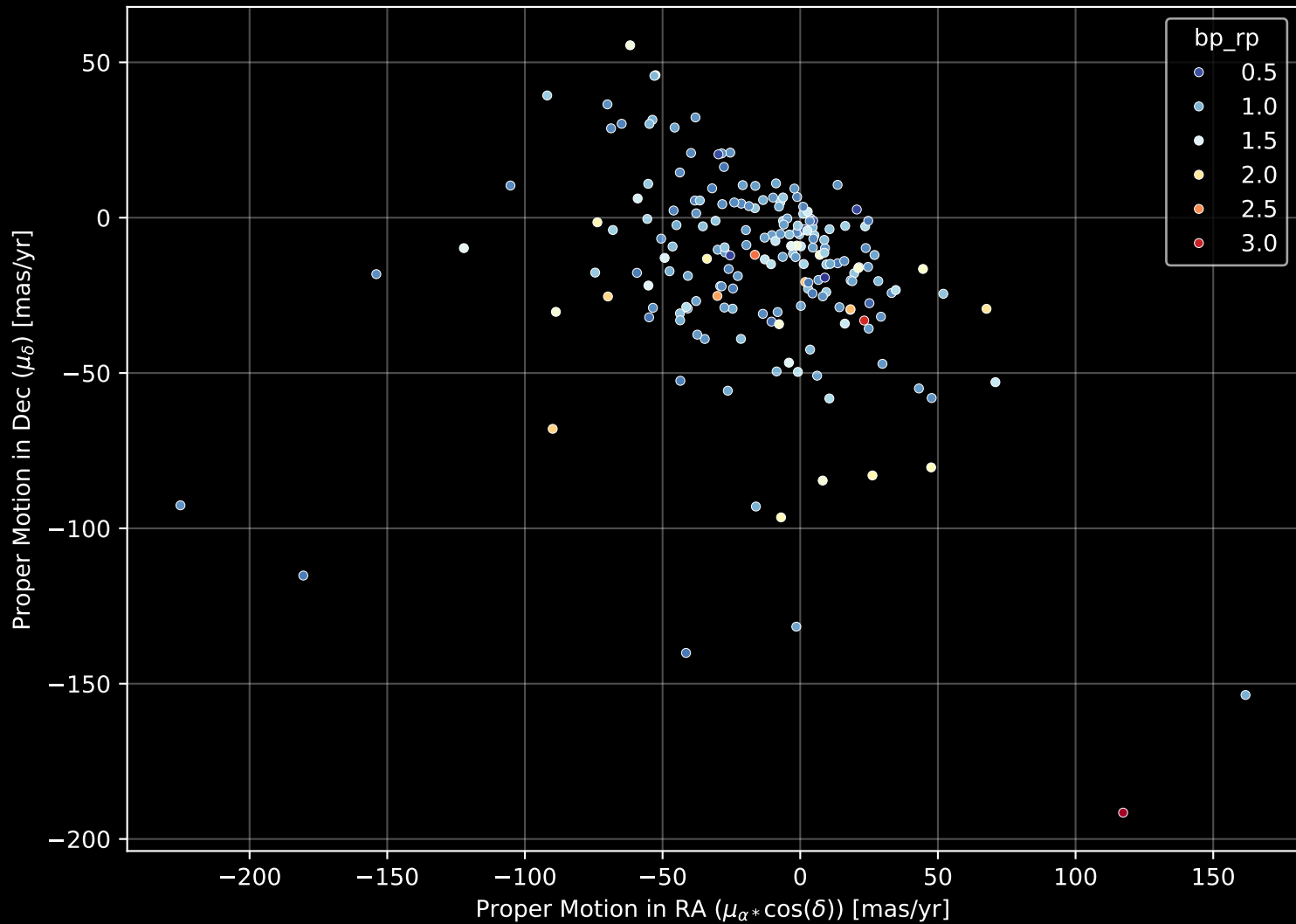
APOGEE DR17 Field: [137+79_MGA] Proper Motion Diagram (n= 191)
