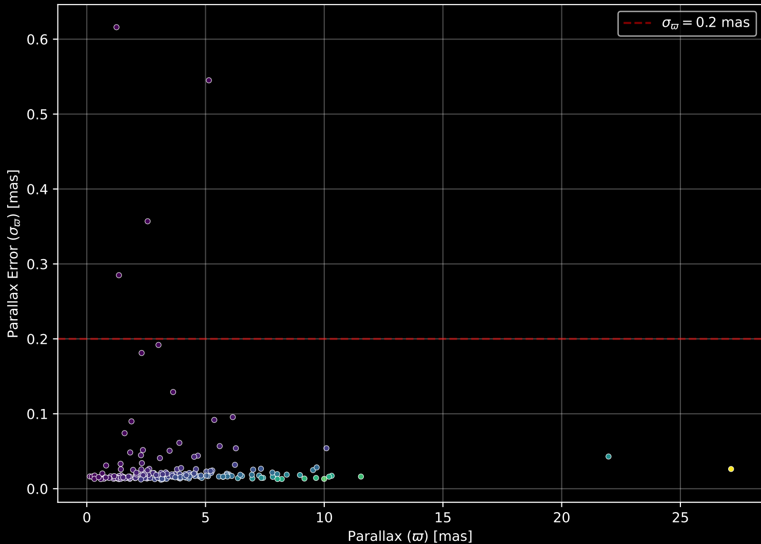
APOGEE DR17 Field: [137+79_MGA] Parallax Quality (n= 191)
