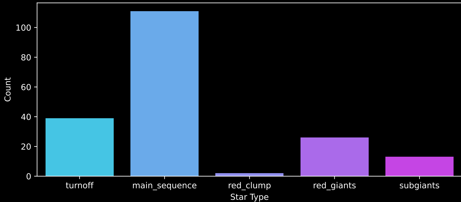
APOGEE DR17 Field: [137+79_MGA] Count plot of Star Type
