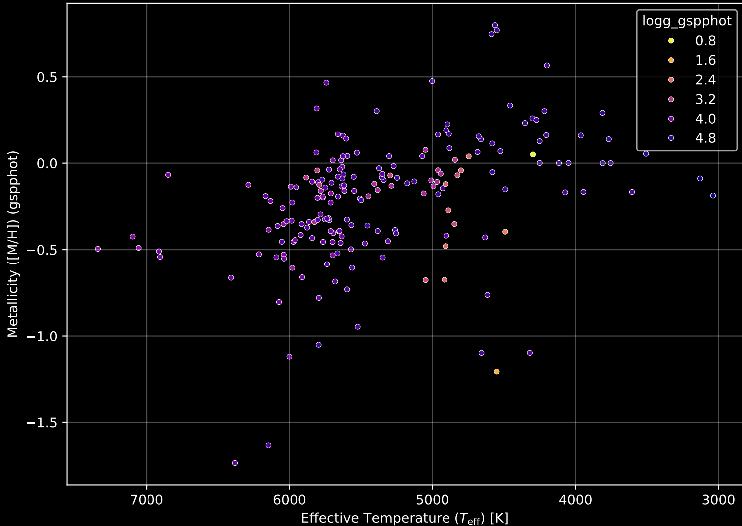
APOGEE DR17 Field: [137+79_MGA] Stellar Population Parameters (n= 191)
