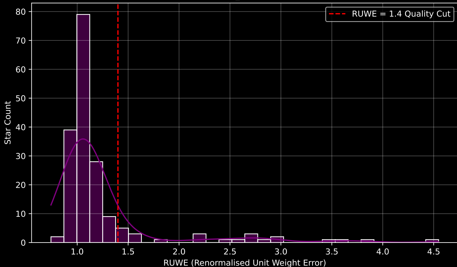
GAPOGEE DR17 Field [137+79_MGA] RUWE Distribution (n= 181)
